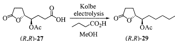
Scheme 9. Kolbe electrolysis of lactono acid ( R,R )- 27 and butanoic acid
