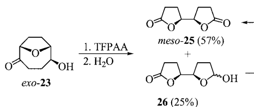
Scheme 7. Baeyer–Villiger oxidation of exo - 23 and subsequent Jones oxidation
