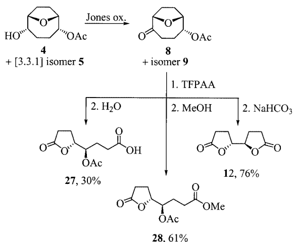
Scheme 8. Baeyer–Villiger oxidation of acetoxy ketones 8 and 9 leading either to bislactone 12 , lactono acid 27 or methyl ester 28
