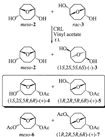
Scheme 2. Synthesis of a mixture of enantiopure monoacetates 4 and 5 by lipase-catalyzed esterification
