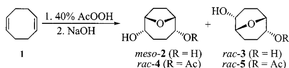
Scheme 1. Synthesis of racemic monoacetates 4 and 5 as well as diols 2 and 3 by transannular O -heterocyclization
