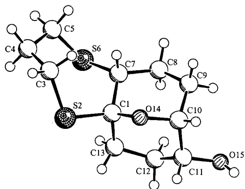
Figure 1. X-ray structure of (1 S ,7 R ,10 R ,11 R )-11-hydroxy-14-oxa-2,6-dithiatricyclo[8.3.1.0 1,7 ]tetradecane (1 S ,7 R ,10 R ,11 R )-( 14 )
