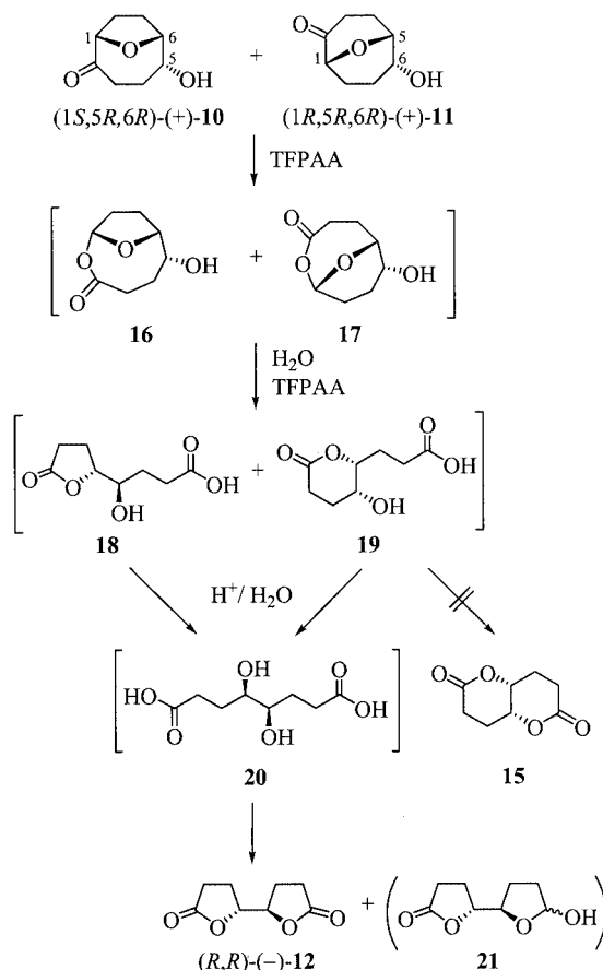
Scheme 5. Presumed mechanism of Baeyer–Villiger oxidation of hydroxy ketones endo -10 and endo -11 leading to 12 as the major product
