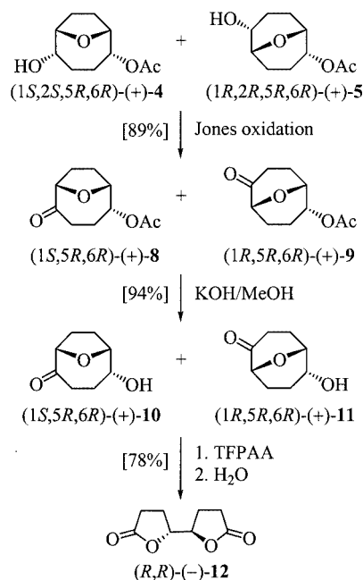
Scheme 3. Reaction sequence leading to bislactone 12
