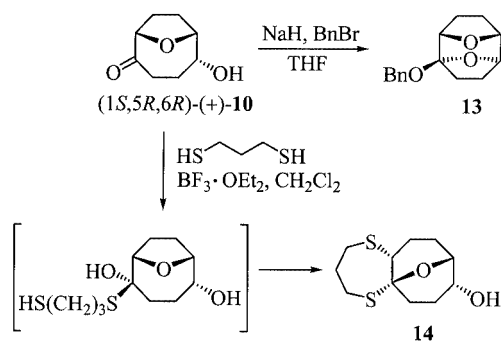
Scheme 4. Derivatizations of hydroxy ketone 10
